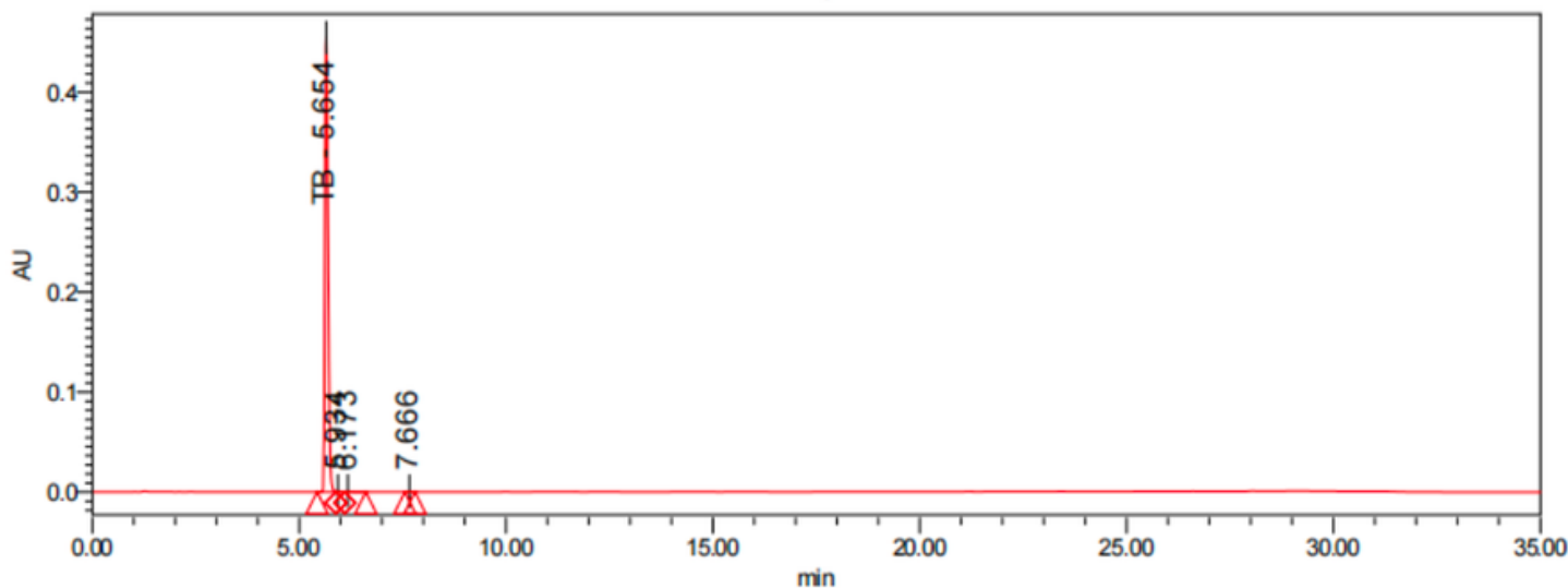
Chromatogram
